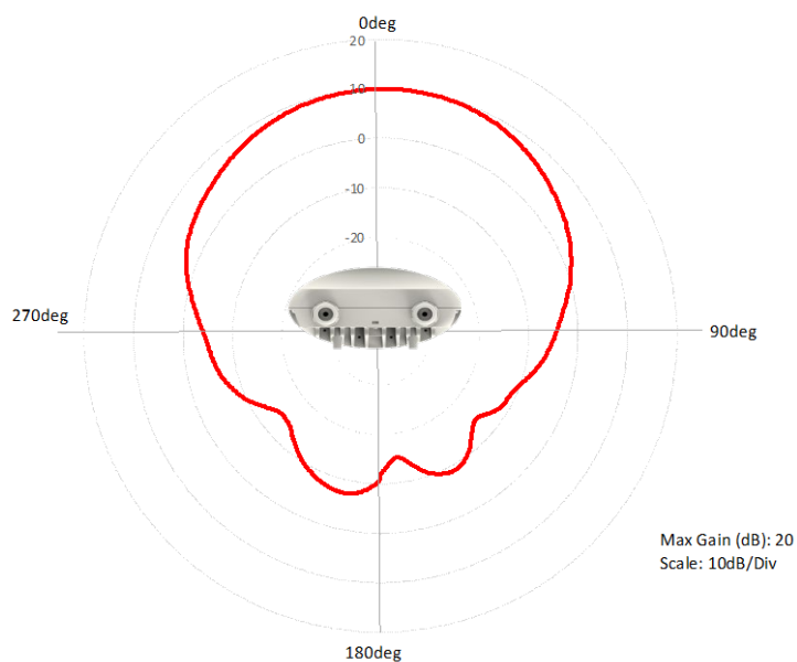
2.4 GHz Azimuth
