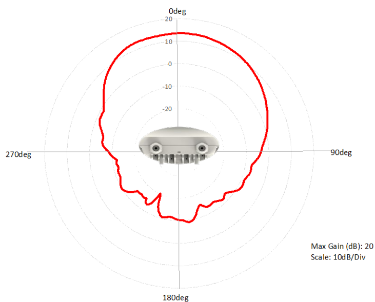
5 GHz Azimuth
