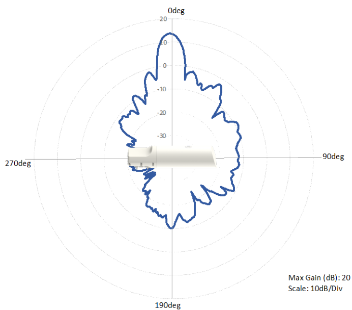
5 GHz Elevation
