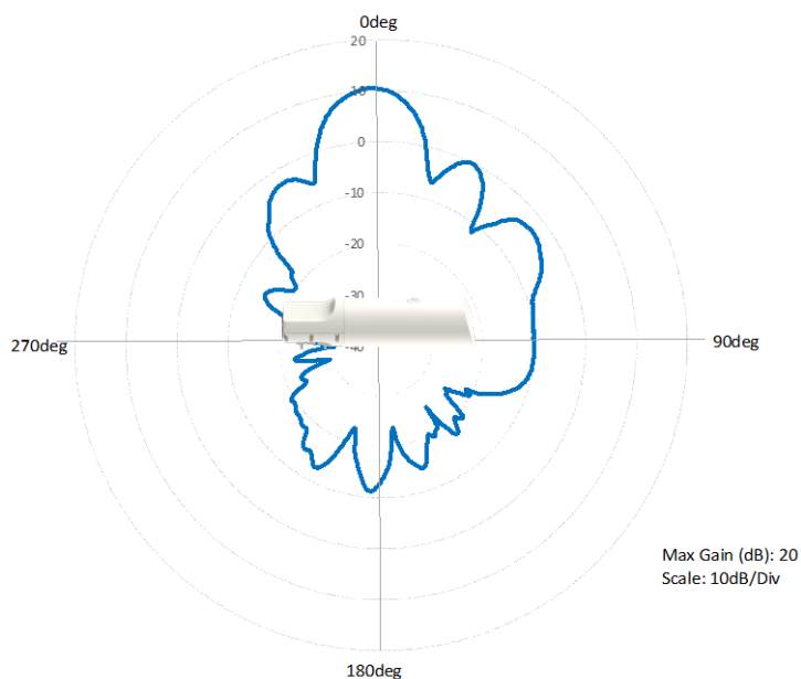
2.4 GHz Elevation
